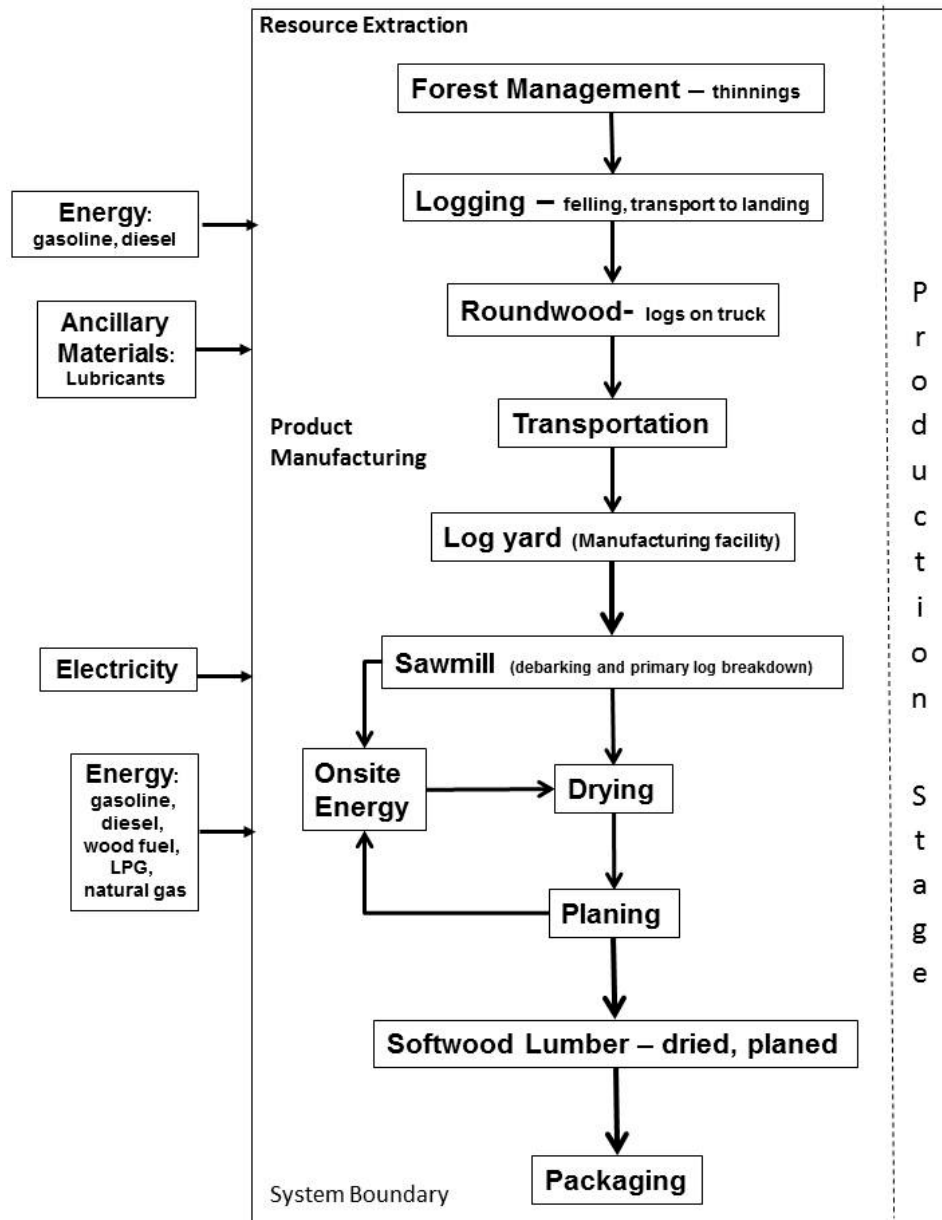
Figure 2 Cradle to gate life cycle stages for softwood lumber production, NE-NC
