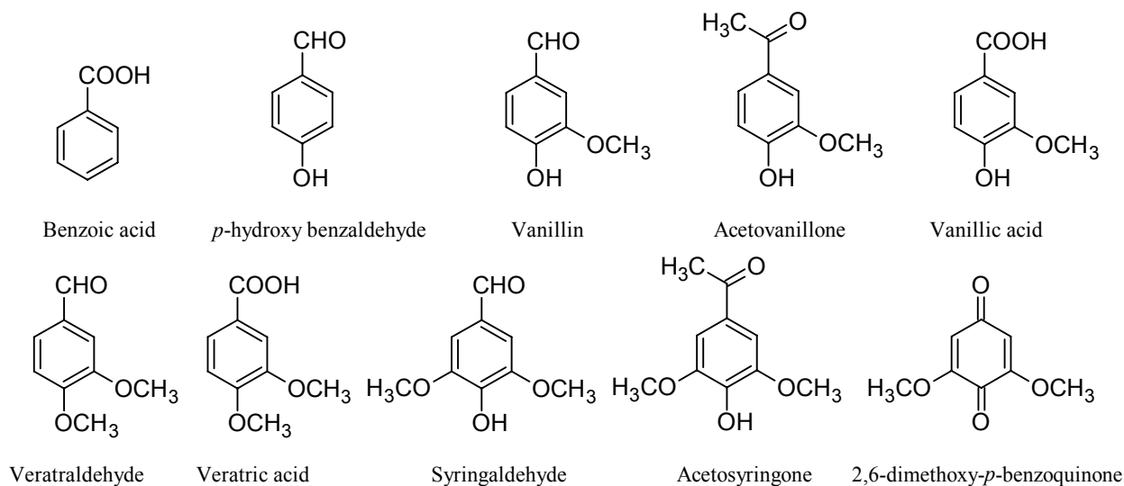
Figure 6. Low-molecular weight compounds identified in softwood and birch kraft pulp POM solution [32].
