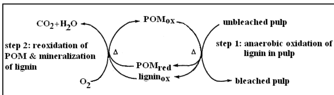
Figure 4. Two steps in POM bleaching.
