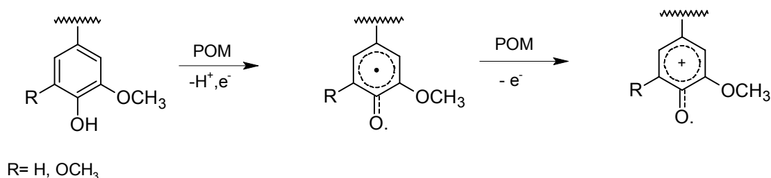
Figure 5. Proposed pathway for formation of the cyclohexadienyl cation upon oxidation of a phenolic lignin model compound by two equivalents of POMs [25].
