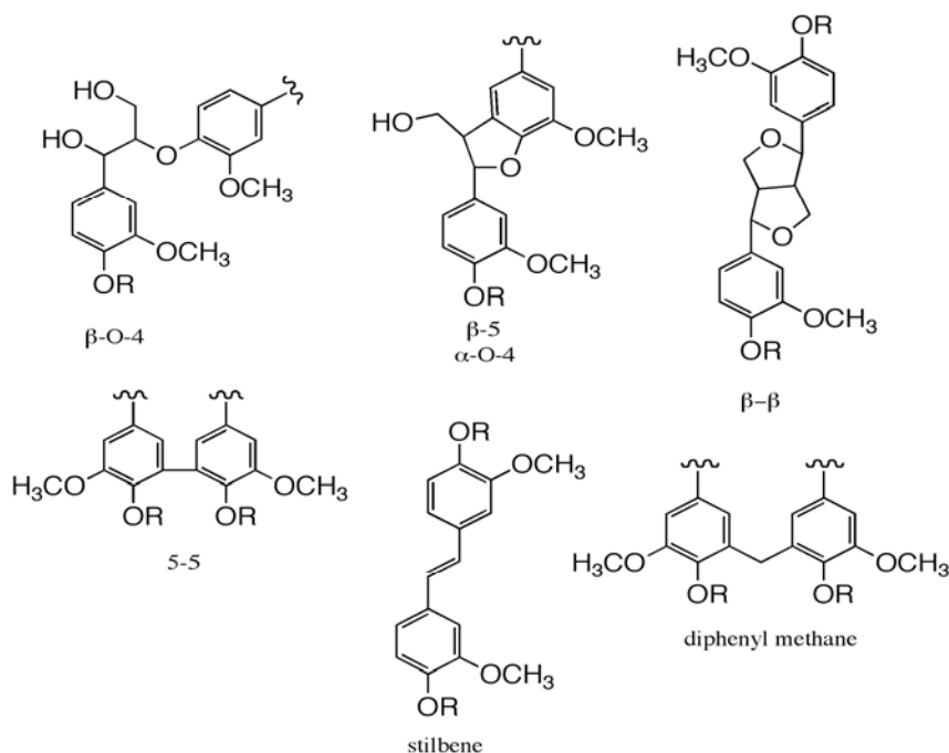
Figure 2. Illustrations of typical softwood lignin structures; \beta -O-4, \beta -5, \alpha -O-4, \beta - \beta and 5-5, additionally, for residual lignin stilbene and diphenylmethane structures. R=H (non-etherified structure); R = Lignin (etherified structure).
