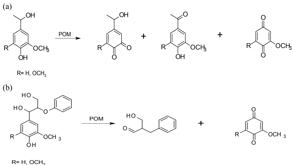
Figure 7. Quinonoid and aromatic products of POM treatment of phenolic LMCs: (a) monomers; and (b) dimers containing \beta -O-4 bond [25,27].
