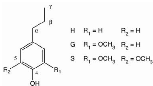
Figure 1. Lignin phenylpropanoid units.
