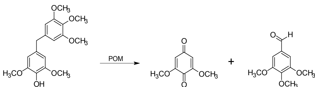
Figure 8. Degradation of a phenolic diphenylmethane with POMs [25].
