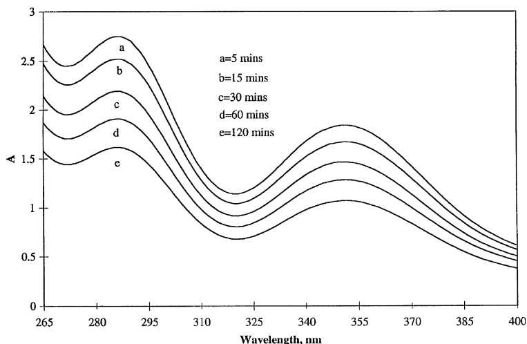
Figure 5. I_3^- concentration decreased after CaCl_2 was added to I_2 + KI solution.
