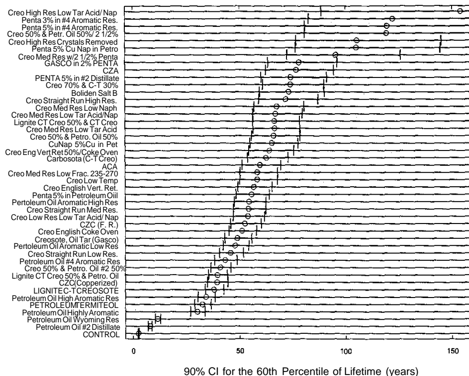
Figure 2. 90% confidence intervals for the 60 th percentile of lifetime of posts impregnated with various treatments.
