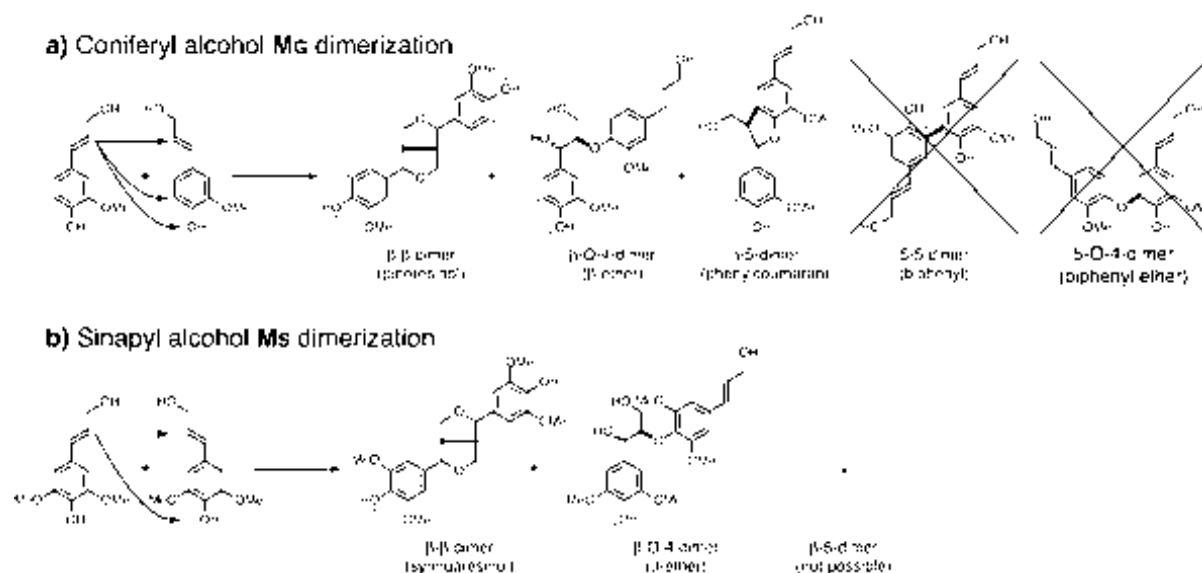
Figure 2. Dehydrodimerization of monolignols. (a) Dehydrodimerization of coniferyl alcohol Me produces only three dimers, in each of which at least one of the coniferyl alcohols is coupled at its \beta -position. The 5-5- and 5-O-4-dehydrodimers shown in most texts (and crossed out in this figure) do not actually arise in any significant way from monolignol dehydrodimerization reactions. The new bond formed by the coupling reaction is bolded. (b) Sinapyl alcohol Ms analogously dehydrodimerizes to only two products.
