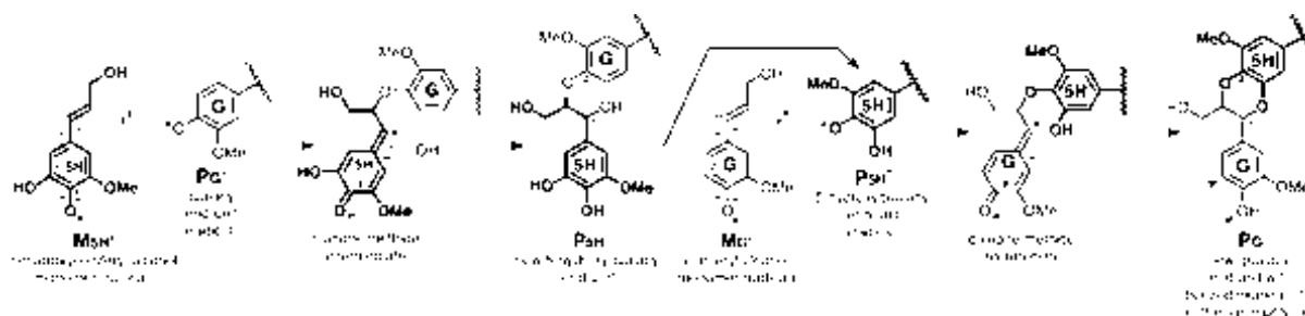
Figure 13. Mechanism of 5-hydroxyconiferyl alcohol M 5H incorporation into a guaiacyl lignin, producing novel benzodioxane units J in the polymer. Only the pathways producing \beta -ether units are shown, but \beta -5- (phenylcoumaran) units are also possible. Cross-coupling with syringyl units is also possible but is less pronounced in lignins which have a low syringyl content due to strong COMT downregulation. Cross-coupling of 5-hydroxyconiferyl alcohol M 5H , via its radical M 5H • , with a guaiacyl lignin unit P G , via its radical P G • , produces a quinone methide intermediate which re-aromatizes by water addition to give the \beta -ether structure possessing a 5-hydroxyguaiacyl end-unit P 5H . This unit is capable of further incorporation into the lignin polymer via radical coupling reactions of radical P 5H • . Reaction with the monolignol coniferyl alcohol M G , via its radical M G • , produces a quinone methide intermediate again. This time, however, the quinone methide can be internally trapped by the 5-OH, forming a new 5-O- \alpha -bond, and creating the benzodioxane ring system. The presence of benzodioxane structures J in COMT-deficient transgenic plants is diagnostically revealed by NMR (Figure 10d2).
