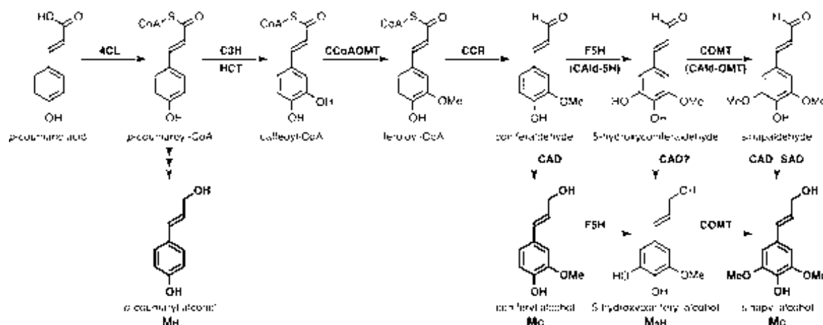
Figure 12. Simplified monolignol biosynthetic pathway. Note that, at least in Arabidopsis, the C3H/HCT conversion involves more steps (Boerjan et al., 2003). Traditional names for the enzymes involved are: 4CL = 4-coumarate:CoA ligase; C3H = p -coumarate 3-hydroxylase; HCT = p -hydroxycinnamoyl-CoA: quinate shikimate p -hydroxycinnamoyltransferase; CCoAOMT = caffeoyl-CoA O-methyltransferase; CCR = cinnamoyl-CoA reductase; F5H = ferulate 5-hydroxylase; CAld5H = coniferaldehyde 5-hydroxylase; COMT = caffeic acid O-methyltransferase; AldOMT = (5-hydroxyconifer)aldehyde O-methyltransferase; CAD = cinnamyl alcohol dehydrogenase. As noted here and in a recent review (Boerjan et al., 2003), many of these enzymes are no longer thought to function on the substrates for which they were originally named.
