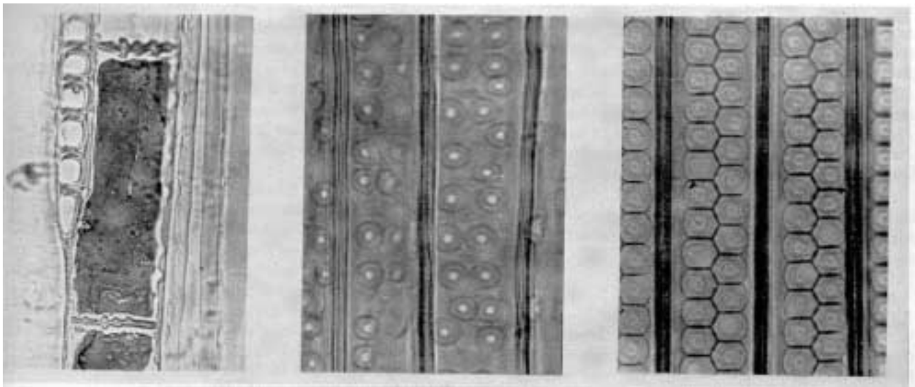
Fig. 3. Left, nodular thickenings of the transverse walls of vertical parenchyma in Taxodium ; Note dark colored contents. Center, bordered pitting of tracheids multiserial and opposite in Sequoia . Right, bordered pitting multiserial and alternate in Agathis
