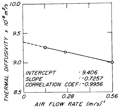
Figure 7.—Determination of true thermal diffusivity of packaged margarine. Extrapolation of data to 0 (m/s) gives thermal diffusivity for a perfectly mixed heat source or sink which is the true thermal diffusivity of the product.
