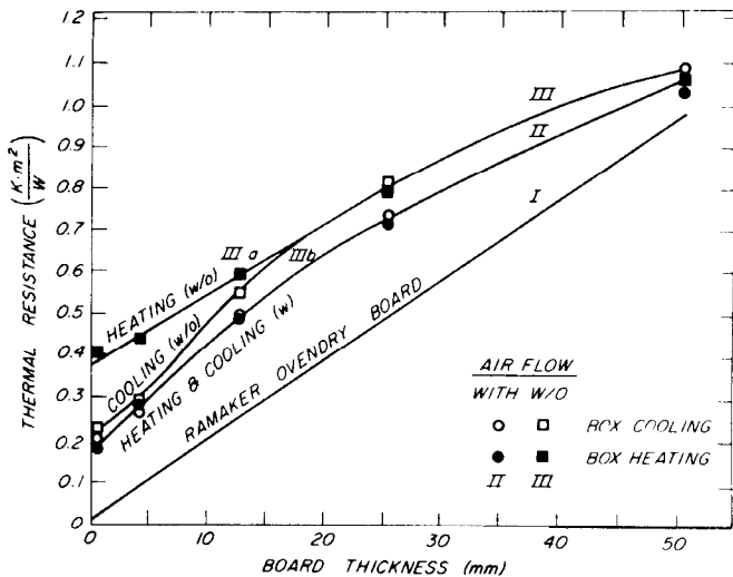
Figure 1.—Overall effective thermal resistance of a cubical corrugated container versus board thickness. Line I is resistance of ovendry board only. Line II is resistance of moist (10 pct moisture) board plus product-container interfacial resistance. Line III is resistance of moist board plus product-container interfacial resistance plus outer bulk air-container interfacial resistance. Line III-a is for heating of the container. Line III-b is for cooling the container.
