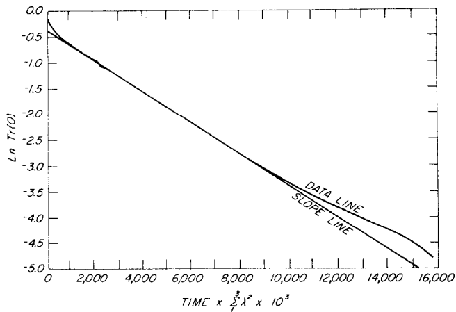
Figure 5.—Determination of the apparent thermal diffusivity of the packaged product (margarine). The "Slope" line approximates the linear region of the "Data" line. The apparent thermal diffusivity of the margarine equals the absolute value of this slope.
