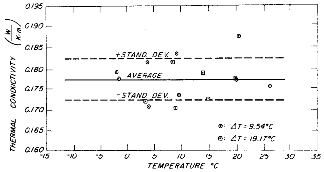
Figure 6.—Thermal conductivity of boxed margarine using a guarded hot-plate apparatus. Standard deviation equaled 0.005 W/K•m. Coefficient of variation was 2.8 percent.
