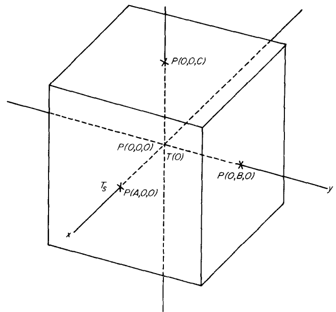
Figure 4.—Rectangular Coordinate system as applied to a package for determination of thermal properties.
