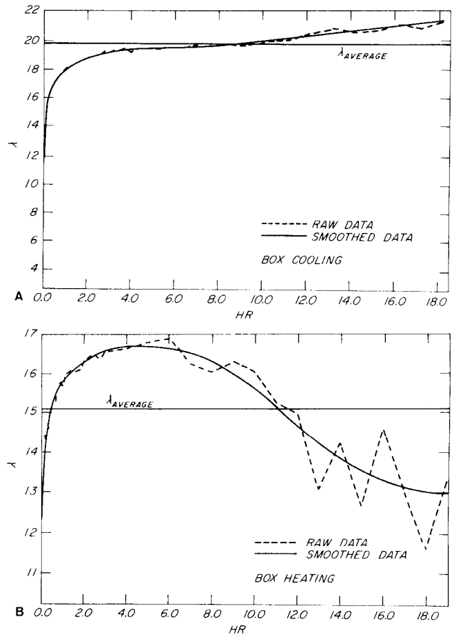
Figure 3.—Change with time of the overall effective heat transfer coefficient (U) as reflected by the first root (1) of the equation U/k = \lambda \tan \lambda L (A) cooling. (B) heating. Horizontal line is the average root found by integrating the area under the smoothed data and dividing by the total time.
