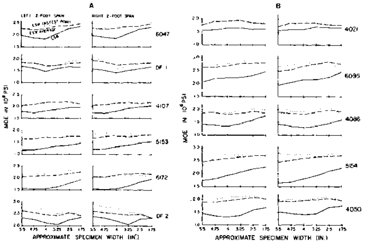
Figure 5.—ESB and ESW based on left end to the hammer and fastest point and average times for the left and right 2-foot portions of the 2-1/2-foot test section containing the knot. A.—Specimen 6047, DF1, 4107, 5153, 6172, and DF2. B.—4021, 6095, 4086, 5154, and 4050.
