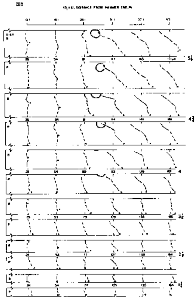
Figure 11.—Specimen 5154. Impact on left end. Estimated stress-wave contours of constant time as specimen width is reduced by ripping. "B" denotes barkside and "P" pithside. Numbers in \mu s represent t . Knots are shown relative to specimen length and width. M 148 976
