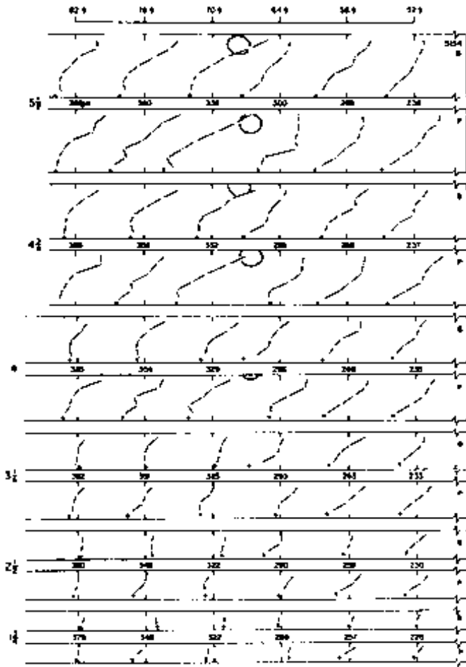
Figure 12.—Specimen 5154. Impact on right end. Estimated stress-wave contours of constant time as specimen width is reduced by ripping. "B" denotes barkside and "P" pithside. Numbers in \mu s represent t . Knots are shown relative to specimen length and width. M 148 977
