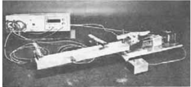
Figure 1.—Stress-wave equipment used to measure transit time (shown with a 2 by 4). (M 141881)
