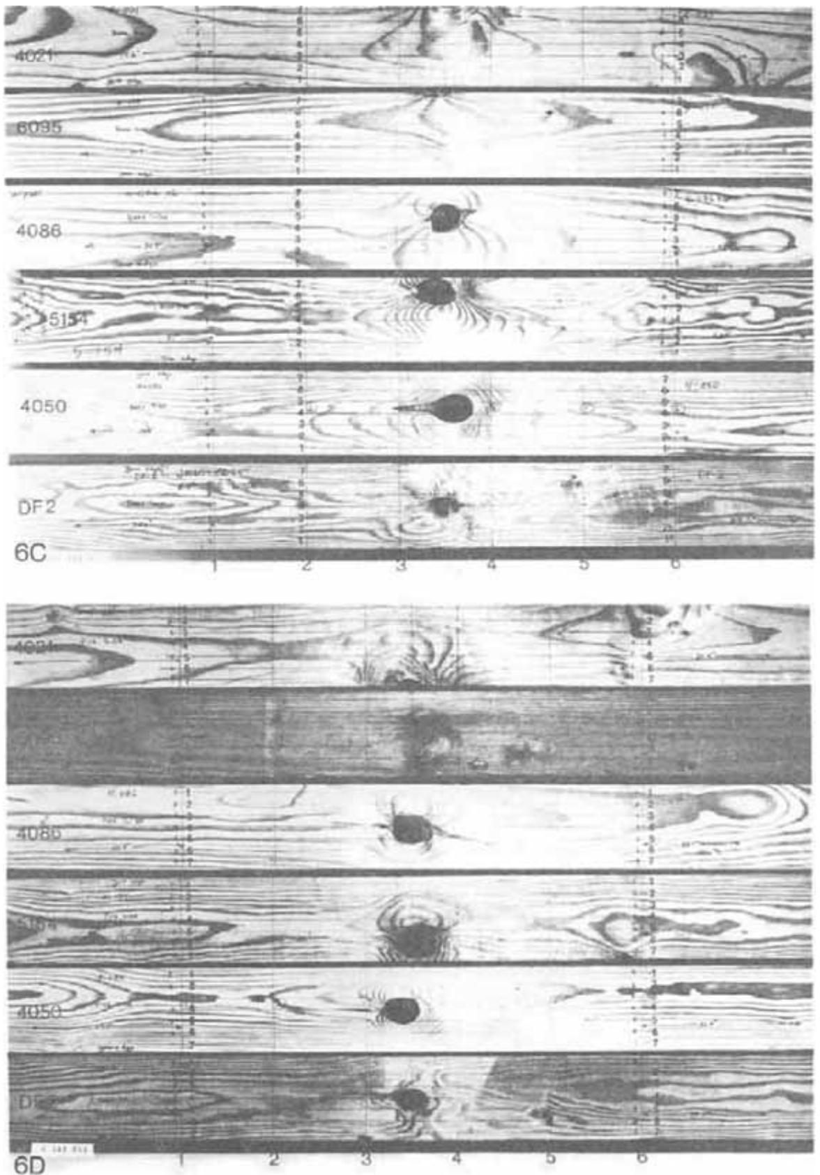
Figure 6 (continued.—Barkside and pithside views of the eleven 8-foot long 2 x 6's. Inscribed on each cross-section are seven 3/4-inch grid lines (type set numbers) and six 6-inch cross-section lines over the 2-1/2-foot test section C. barkside and D. pithside of 4021, 6095, 4086, 5154, 4050, and DF2. M 141 251, M 141 252
