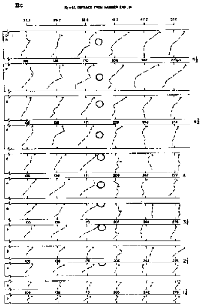
Figure 10.—Specimen DF 1. Estimated stress-wave contours of constant time as specimen width is reduced by ripping. "B" denotes barkside and "P" pithside. Numbers in \mu s represent t . Knots are shown relative to specimen length and width. M 148 975
