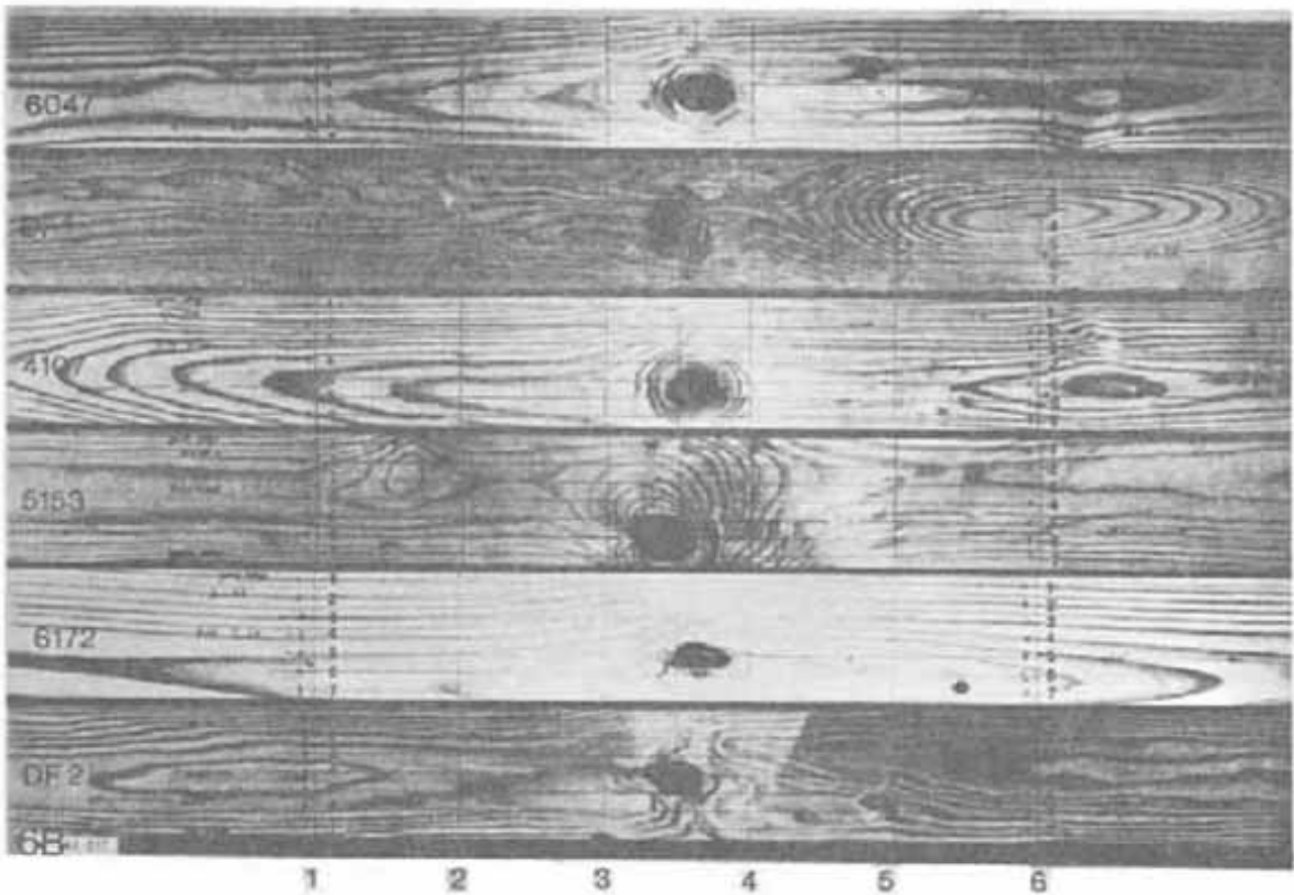
Figure 6.—Barkside and pithside views of the eleven 8-foot long 2 x 6's. Inscribed on each specimen are seven 3/4-inch grid lines (type set numbers) and six 6-inch cross-section lines over the 2-1/2-foot test section. A. barkside and B. pithside of 6047, DF1, 4107, 5153, 6172, and DF2. M 141 254, M 141 253
