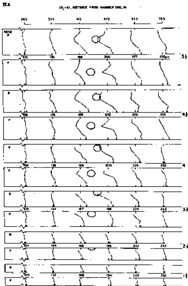
Figure 8.—Specimen 4050. Estimated stress-wave contours of constant time as specimen width is reduced by ripping. "B" denotes barkside and "P" pithside. Numbers in \mu s represent t . Knots are shown relative to specimen length and width. M 148 973
