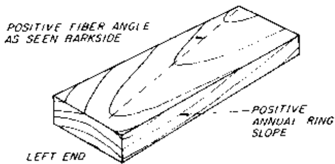
Figure 7.—Schematic showing positive slopes of fiber angle and annual rings. M 148 972
