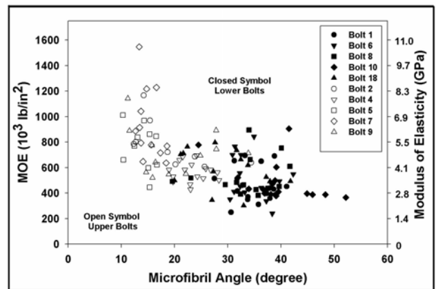
Figure 5—Latewood MOE compared to Microfibril angle.
