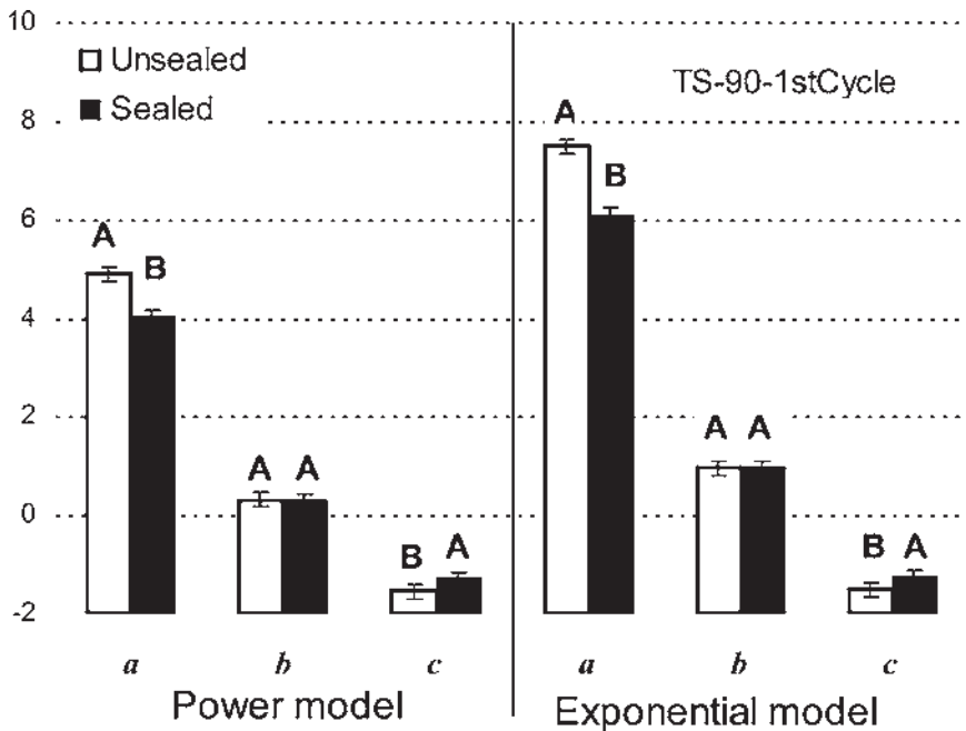
Figure 2. Coefficient values of thickness swelling curve for 90% RH exposure: effect of edge sealing. Values are from the first 90% RH exposure for control specimens (unburnt, 0% bark). Error bars are standard deviations; same letter (upper case) denotes statistically similar results ( \alpha = 0.05 ) between column pairs.
