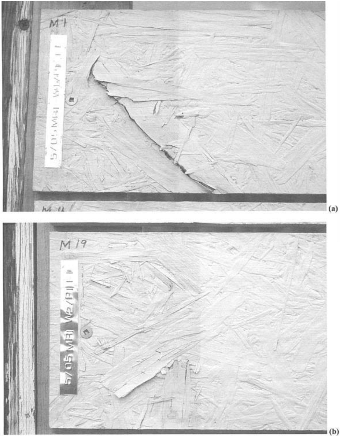
Figure 5. Close-up of boards on the test fence near Madison, Wisconsin, showing deterioration at the edges of large surface flakes.
