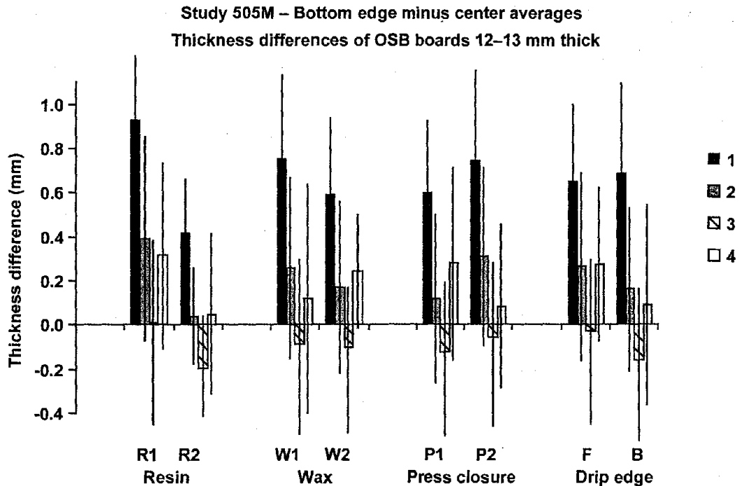
Figure 11. Thickness-swell difference between drip edge and center of board for: unsealed drip edge/one coat of paint (1); unsealed drip edge/ two coats of paint (2); sealed drip edge/two coats of paint (3); and sealed drip edge/one coat of paint (4). Lack of a line indicating first standard deviation indicates all evaluations were the same. R1 is 2.0% resin, R2 is 3.5% resin, W1 is 0.75% wax, and W2 is 1.5% wax. P1 is continuous press closure, P2 is two-stage press closure, F is flat edge, and B is bevel edge.
