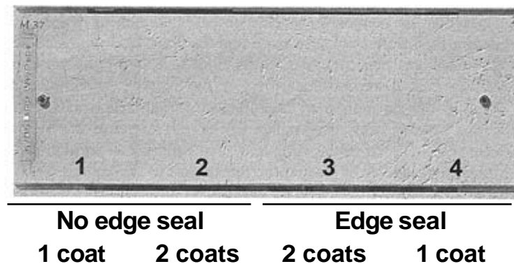
Figure 1. Single board showing four sections: 1. One coat of paint, no edge seal; 2. Two coats of paint, no edge seal; 3. Two coats of paint, edge seal; 4. One coat of paint, edge seal.
