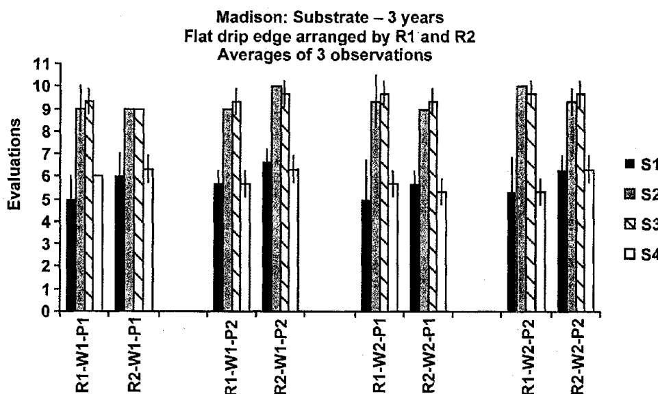
Figure 7. Substrate evaluations following 3 years of exposure near Madison., Wisconsin, for unsealed drip edge/one coat of paint (S1); unsealed drip edge/two coats of paint (S2); sealed drip edge/two coats of paint (S3); and sealed drip edge/one coat of paint (S4). R1 is 2.0% resin, R2 is 3.5% resin, W1 is 0.75% wax, and W2 is 1.5% wax. Error bars indicate \pm one standard deviation from mean. Lack of a line indicating first standard deviation indicates all evaluations were the same.
