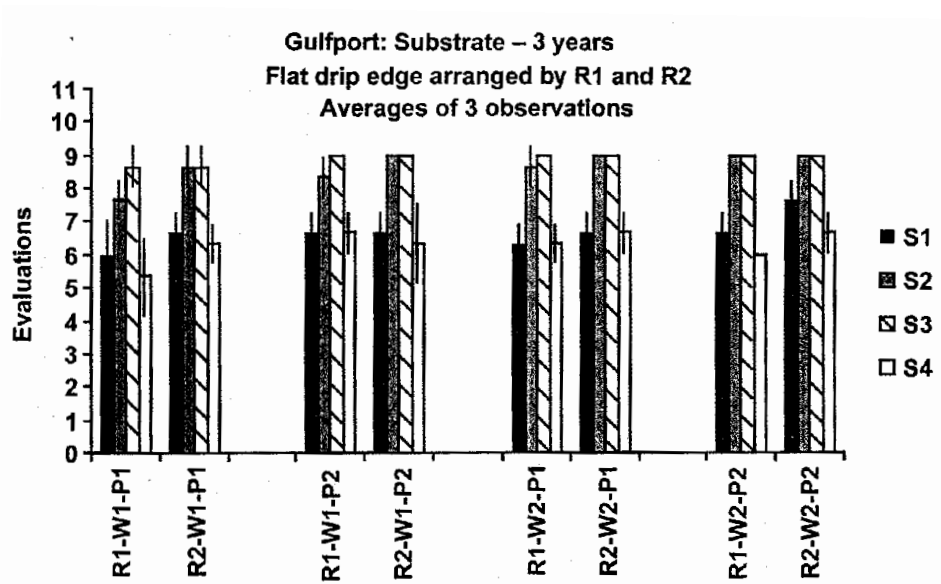
Figure 8. Substrate evaluations following 3 years of exposure near Gulfport, Mississippi, for unsealed drip edge/one coat of paint (S1); unsealed drip edge/two coats of paint (S2); sealed drip edge/two coats of paint (S3); and sealed drip edge/one coat of paint (S4 R1 is 2.0% resin, R2 is 3.5% resin, W1 is 0.75% wax, and W2 is 1.5% wax. Error bars indicate \pm one standard deviation from mean. Lack of a line indicating first standard deviation indicates all evaluations were the same.
