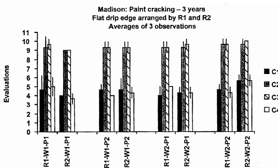
Figure 9. Paint cracking evaluations following 3 years of exposure near Madison, Wisconsin, for unsealed drip edge/one coat of paint (C1); unsealed drip edge/two coats of paint (C2); sealed drip edge/two coats of paint (C3); and sealed drip edge/one coat of paint (C4). R1 is 2.0% resin, R2 is 3.5% resin, W1 is 0.75% wax, and W2 is 1.5% wax. Error bars indicate \pm one standard deviation from mean. Lack of a line indicating first standard deviation indicates all evaluations were the same.
