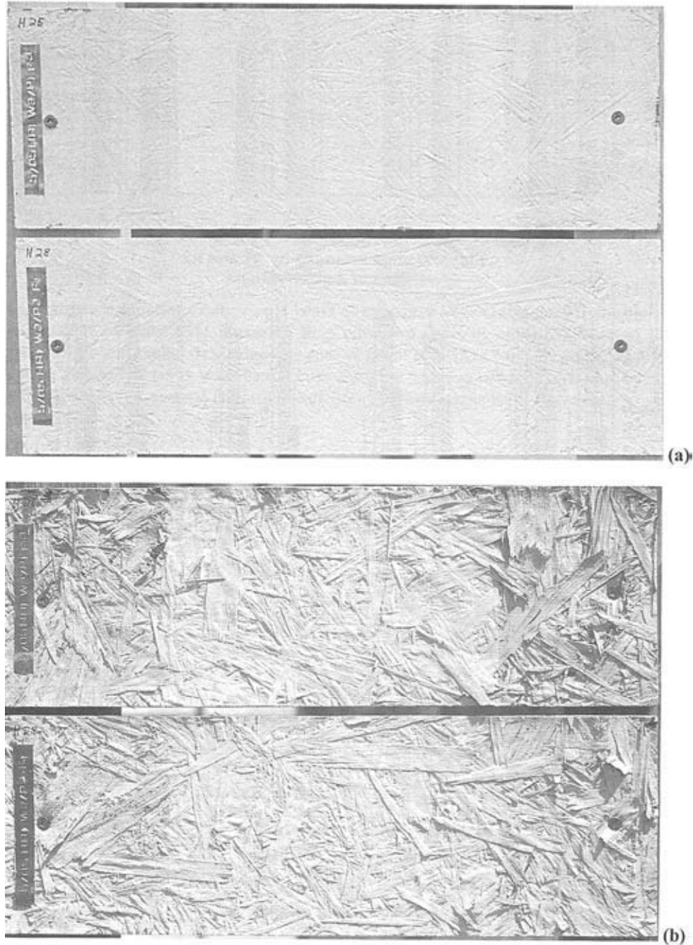
Figure 6. Close up of two boards just after installation (a) on the test fence near Gulfport, Mississippi, and following 3 years of exposure (b).
