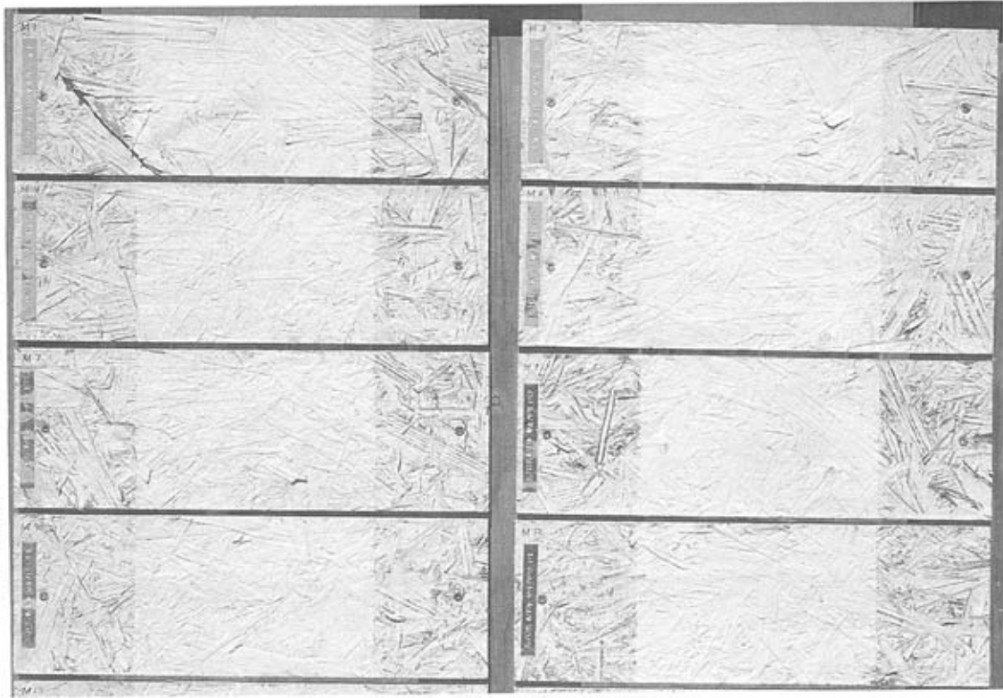
Figure 4. Close-up of the same boards as shown in Figure 3 after 3 years on the test fence near Madison, Wisconsin.
