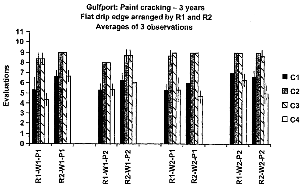
Figure 10. Paint cracking evaluations following 3 years of exposure near Gulfport, Mississippi, for unsealed drip edge/one coat of paint (C1); unsealed drip edge/two coats of paint (C2); sealed drip edge/two coats of paint (C3); and sealed drip edge/one coat of paint (C4). R1 is 2.0% resin, R2 is 3.5% resin, W1 is 0.75% wax, and W2 is 1.5% wax. Error bars indicate 5 one standard deviation from mean. Lack of a line indicating first standard deviation indicates all evaluations were the same.
