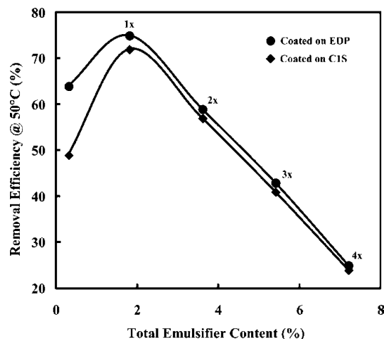
Figure 4. Removal efficiencies for PSA2 coated on EDP and CIS as a function of the emulsifier content. The labels on the data indicate the amount of emulsifier that is part of the latex relative to what is typically used in its synthesis, e.g., 1x is the amount of the emulsifier used in the polymerization and 2x indicates that emulsifier has been added subsequent to synthesis to raise the concentration to twice its typical level in the latex.
