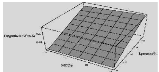
FIG. 6. Model-predicted tangential thermal conductivity values for latewood percentages from 10% to 99% and MC from 0% to 30%.
