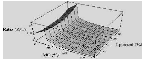
FIG. 11. Ratio of radial versus tangential thermal conductivity values predicted for Scots pine.
