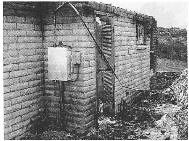
Figure 4. - Vents located on an exterior door possibly contributed to loss of this structure by allowing burning embers into the room containing mechanical equipment.
