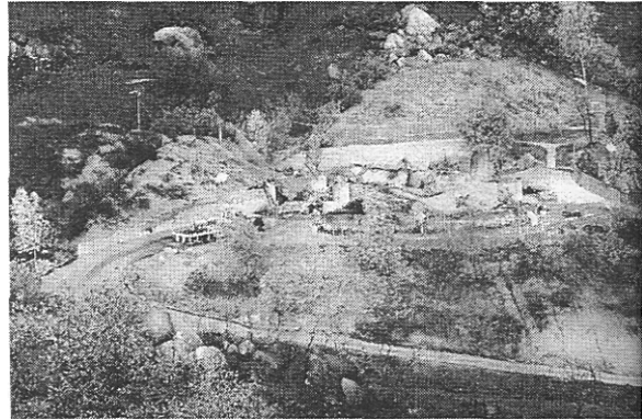
Figure 1. ~ A noncombustible exterior cladding and roof covering, plus dual pane windows were not enough to save this structure. Ember entry into vents are a probably cause of the initial ignition of this structure.
