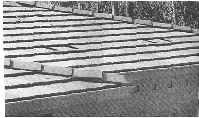
Figure 6. ~ Additional flat through-roof vents, located on the lower portion of a sloped roof used instead of the more traditional soffit or eave vent. Two of these vents can be observed in this photograph. With these vents, entry to the attic space is off-set from the openings to the outside, thereby reducing the potential for entry of rain into the attic space.
