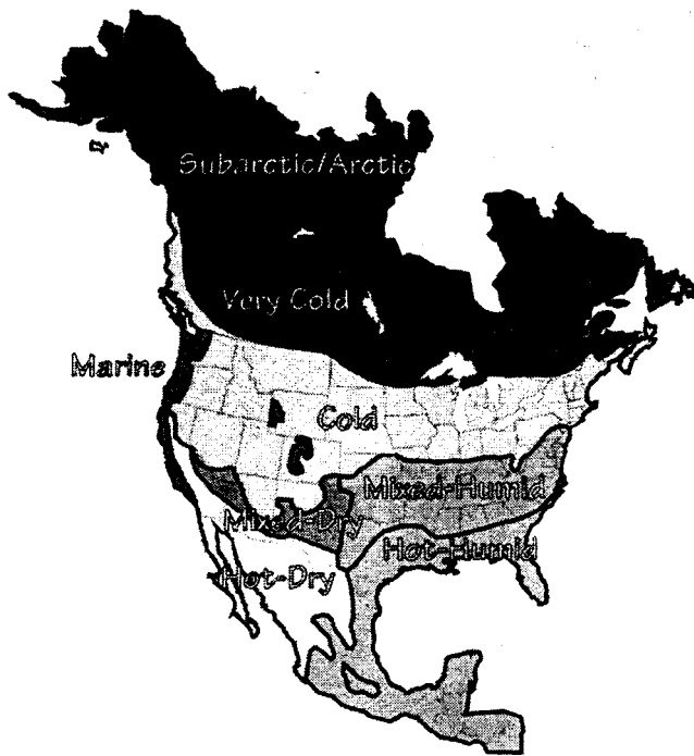
Figure 5. ~ Climate map of North America (courtesy of Joe Lstiburek, Ph.D., Building Science Corporation, Westford, MA).
