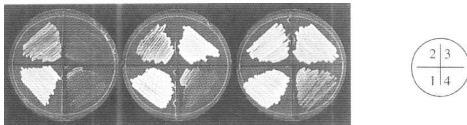
Fig. 2. Growth of FPL-MY30 and its parental strains on various carbon sources. The plates are divided into four sectors by the manufacturer. 1, YNB medium containing 2% glucose; 2, YNB medium containing 2% glycerol; 3, YNB medium containing 2% xylose; 4, YNB medium containing 2% L-arabinose. Uridine (20 mg/L) was supplied in all plates.
