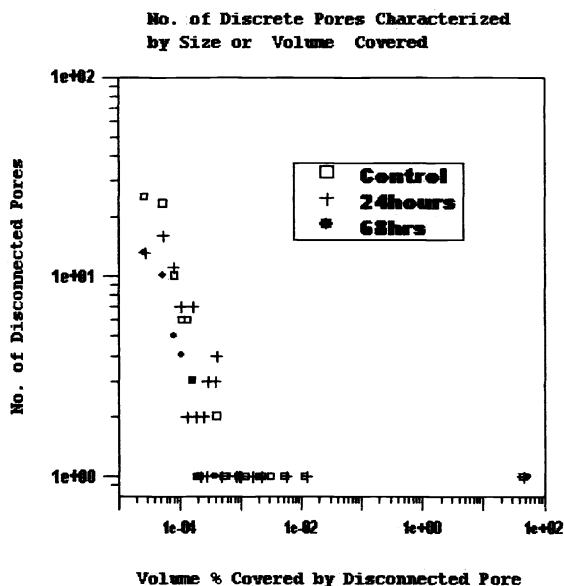
Figure 5. Disconnectivity Curves
