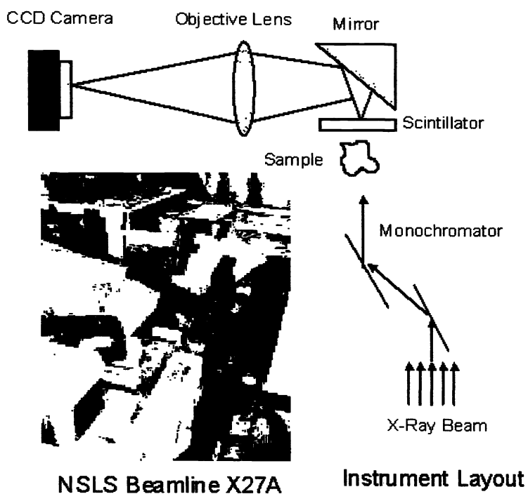
Figure 1. XCMT apparatus
