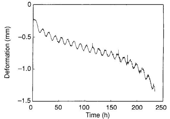
FIG. 2. Deformation varying with time of a short column of corrugated fiberboard subjected to 1.75 kN/m (10 lbf/in.) static edgewise compression and cyclic relative humidity (Fig. 1). The short column was 51 mm (2 in.) wide by 38 mm (1.5 in.) high, with height in the axis direction of the flutes. The region of secondary creep lies approximately between 50 h and 150 h.
