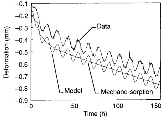
FIG. 7. Comparison between subset of deformation varying with time data (Fig. 2) and plot of Eq. (20) fit to the data. Vertical scale of deformation data is offset for clarity.
