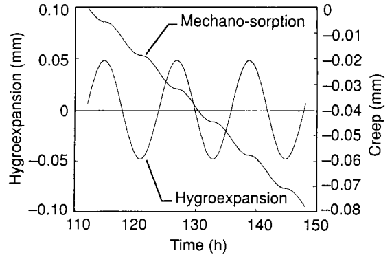
FIG. 4. Comparison over time between the hygroexpansion of a short column of corrugated fiberboard subjected to cyclic RH and the mechano-sorption caused by static compression and the hygroexpansion. Hygroexpansion is plotted with A_0 = 0 .
