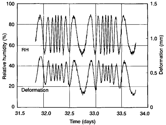
FIG. 8. Upper curve: Relative humidity compared with time from Fig. 2. Lower curve: Variation of deformation of corrugated fiberboard tube with time when subjected to humidity excitation.
