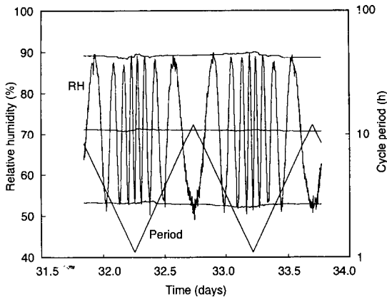
FIG. 2. Variation of relative humidity with time following swept sine control signal. Lines through approximate steady-state, maximum, and minimum values represent moving window, three-cycle band width fit to data of swept sine wave defined by p_t = 12 , target p_t = 1 , target P_s = 24 , and R_d = 1/2 .
