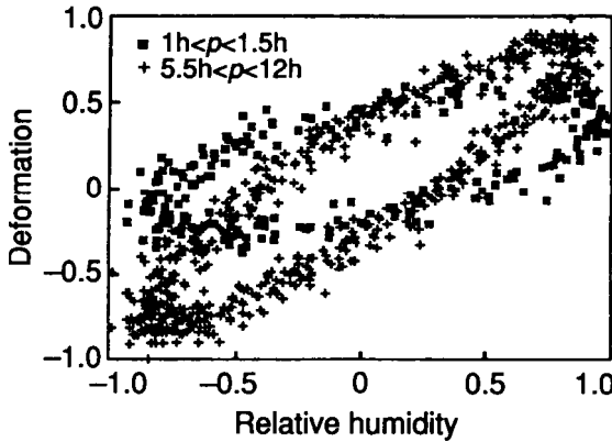
FIG. 9. Lissajous diagram of data with form shown in Fig. 8. Scales are normalized with respect to \pm 1 .
