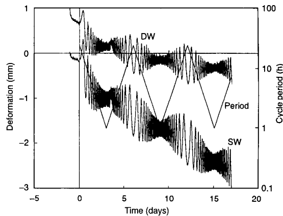
FIG. 5. Variation of deformation of single-walled (SW) and double-walled (DW) corrugated fiberboard tubes with time, when subjected to static load equal to 17% of tube compression strength and swept sine relative humidity excitation.
