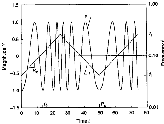
FIG. 1. Swept sine wave with p_i = 24 , target p_t = 4 , target P_s = 48 , and \omega = -1/2 in which frequency varies logarithmically with time so that frequency change per cycle remains constant.
