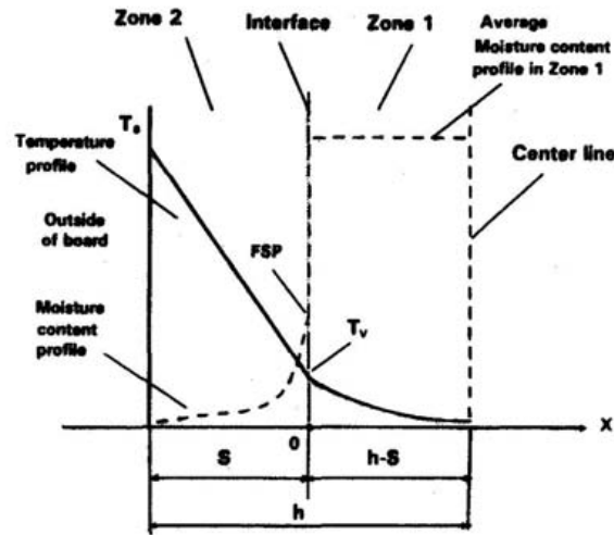
FIG. 1. Model for heat transfer and retreat of interface in the press-drying process.
