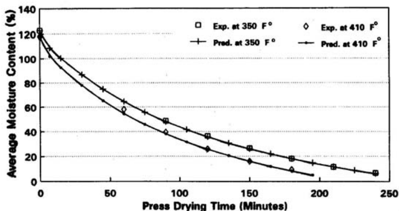
FIG. 2. Comparison of predicted (Pred.) and experimental (Exp.) curves for the drying temperatures 350 F and 410 F. (each point is an average value of 12 boards)
