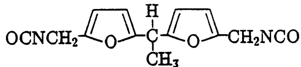
Figure 1 Chemical structure of EDFI.
