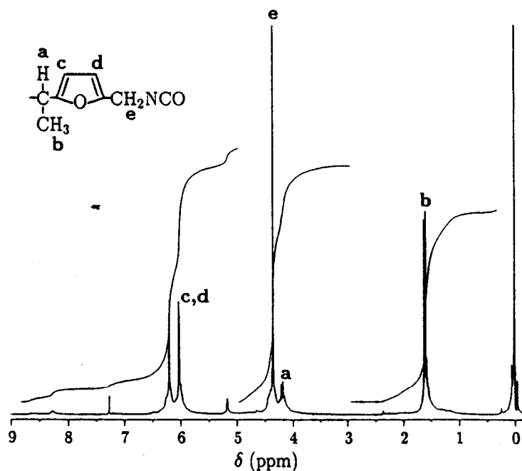
Figure 3 1 H-NMR spectrum of EDFI.
