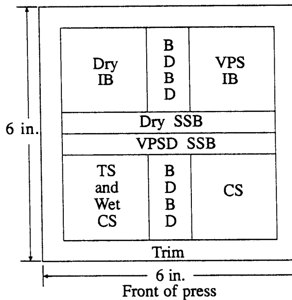
Figure 6 Pattern used for cutting test specimens from the Bakeboards. The type of test performed on each specimen is indicated as follows: IB is internal bond; BDBD is boil-dry-boil-dry; SSB is small specimen bending; TS is thickness swell; CS is compression shear (1 in. = 25.4 mm).
