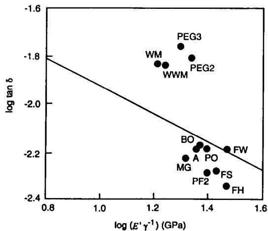
FIG. 7. Relationships between logarithm of E'/\gamma and logarithm of \tan \delta for chemically modified wood at 35% relative humidity. (Line on graph from Fig. 3.)
