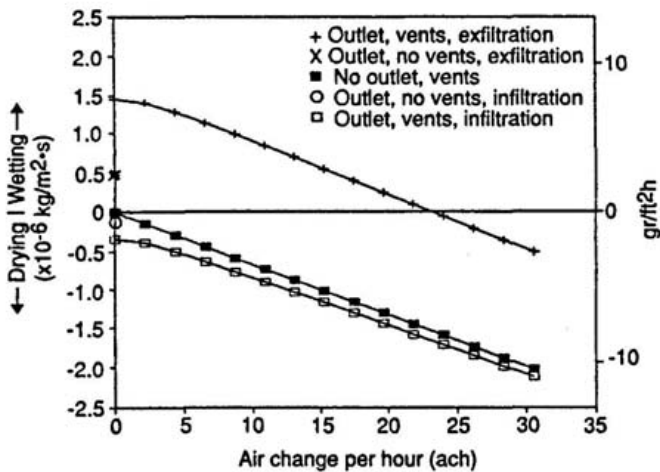
Figure 5 Influence of vents, electrical outlets, and airflow on wetting and drying potential in wood-Same wall during winter.
