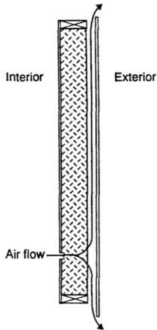
Figure 6 Purely exfiltrative airflow in wall.
