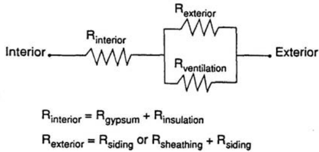
Figure 3 Model for heat or vapor transfer through wall.
