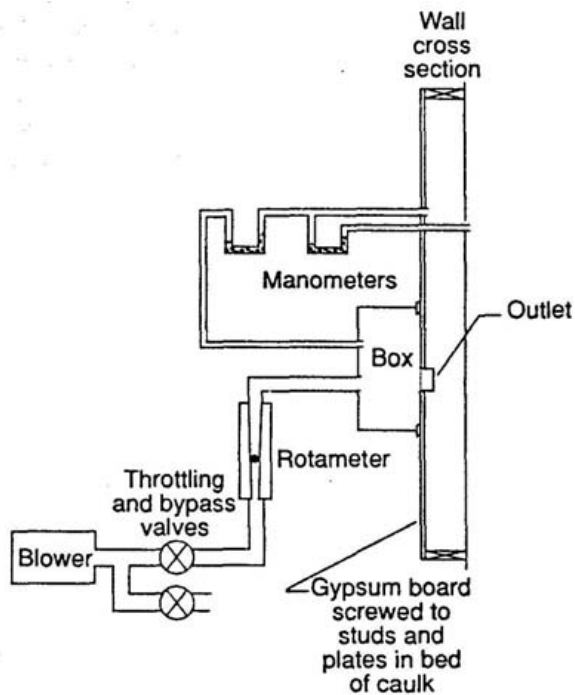
Figure 4 Apparatus used to measure airtightness of walls with electrical outlets (box shown was pressurized).
