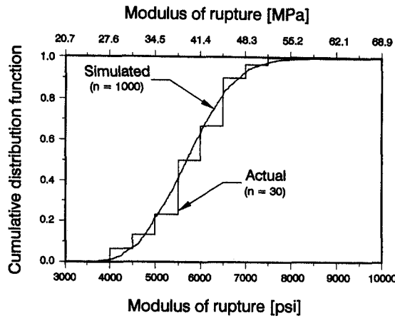
FIG. 1. Simulated and actual cumulative distribution functions of beam modulus of rupture.
