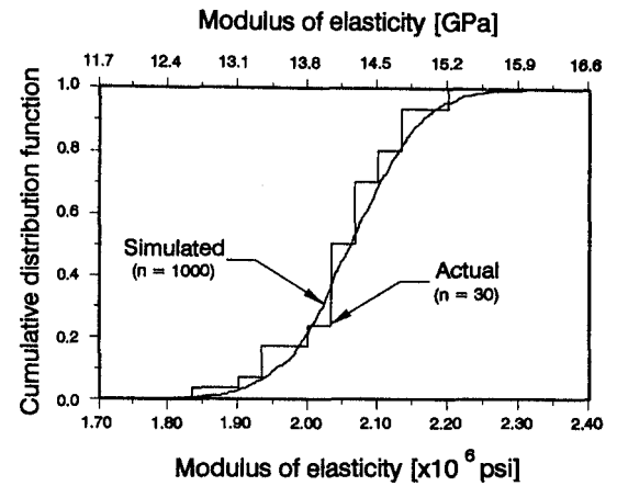
FIG. 2. Simulated and actual cumulative distribution functions of beam modulus of elasticity.
