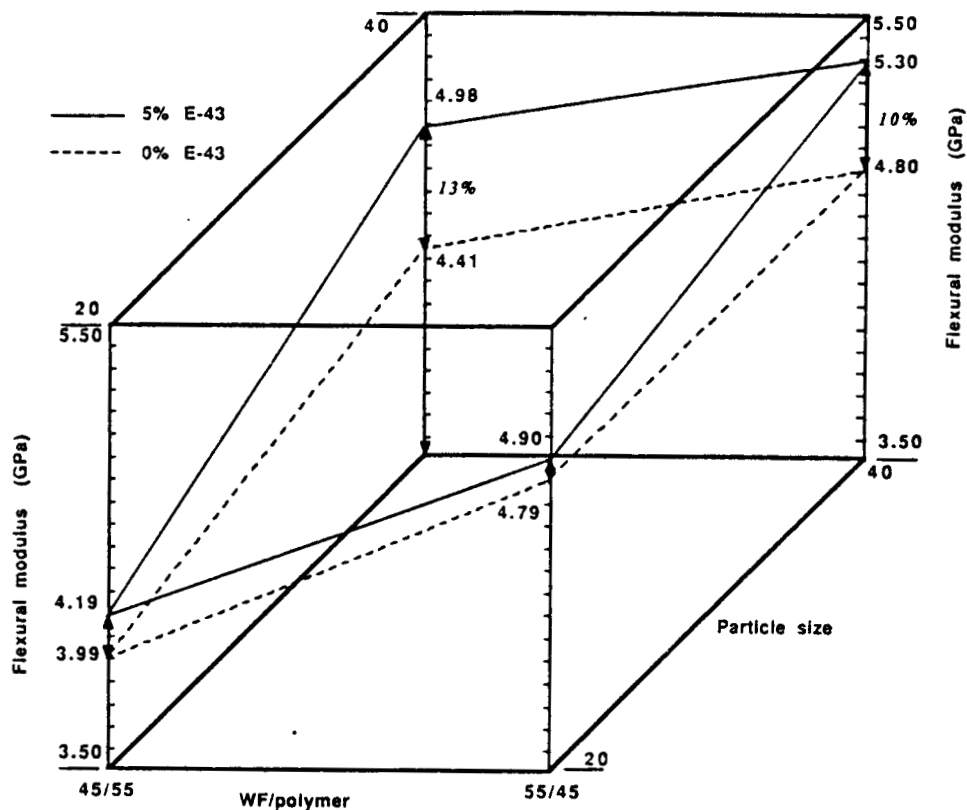
FIGURE 8 Flexural modulus as a function of wood flour to total polymer weight ratio, wood flour particle size, and Epolene E-43 content. (All data points are the average of results for one and three extrusions. Epolene E-43 levels are weight percentages of wood flour.)
