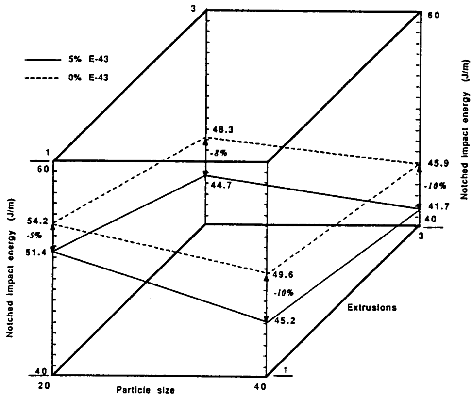
FIGURE 10 Notched impact energy as a function of wood flour particle size, number of extrusions, and Epolene E-43 content. (All data points are the average of results for one and three extrusions. Epolene E-43 levels are weight percentages of wood flour.)
