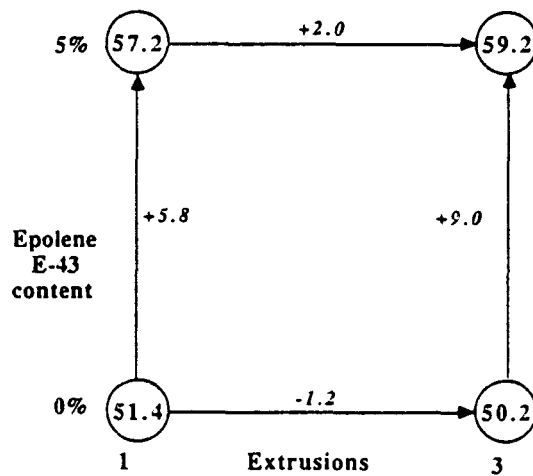
FIGURE 2 Two-factor interaction between Epolene E43 content (0 or 5 percent) and number of extrusions (1 or 3) for maximum cantilever-beam strength in megapascals. (Significant at 90 percent confidence limit).
