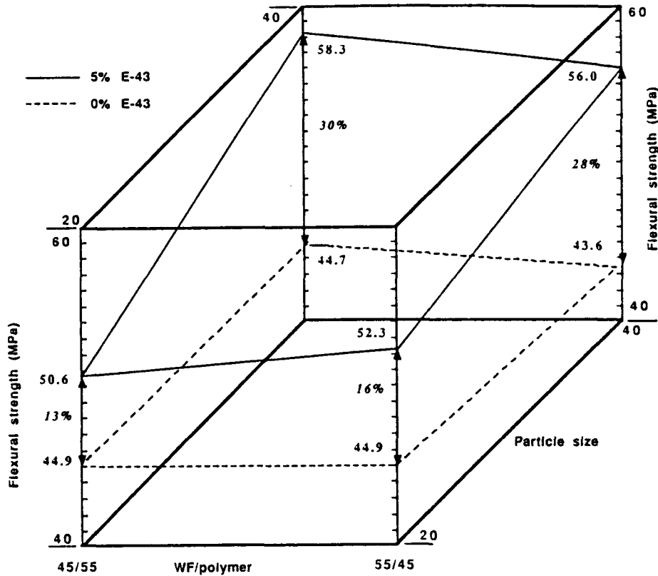
FIGURE 4 Maximum flexural strength as a function of wood flour to total polymer weight ratio (WF/polymer), wood flour particle size, and Epolene E-43 content. (All data points are the average of results for one and three extrusions. Epolene E-43 levels are weight percentages of wood flour.)
