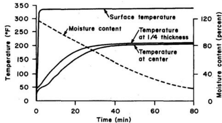
FIG. 1. Changes in temperature and moisture content of 1.60-in.-thick loblolly pine during press drying at 25 lb/in. 2 and 350 F. (ML89 5650)
