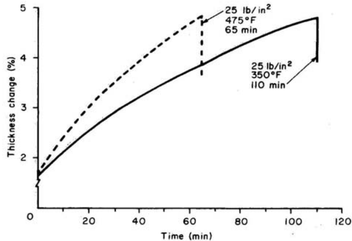
FIG. 7. Thickness change of 1.75-in.-thick loblolly pine during press drying. (ML89 5569)
