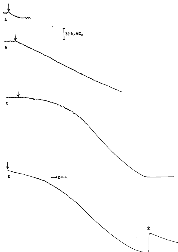
FIGURE 4: Oxygen consumption in LiP reactions in oxalate buffer. Reaction mixtures contained 10 mM oxalate, pH 3.0, 0.1 unit/mL LiP, and 50 μM veratryl alcohol. Arrows indicate addition of H 2 O 2 . (A) Standard reaction mixture, 50 μM H 2 O 2 ; (B) plus 1 mM MnSO 4 , 50 μM H 2 O 2 ; (C) same conditions as in (B) but with 5 μM H 2 O 2 ; (D) same conditions as in (C), asterisk indicates addition of 9.3 units/mL catalase.
