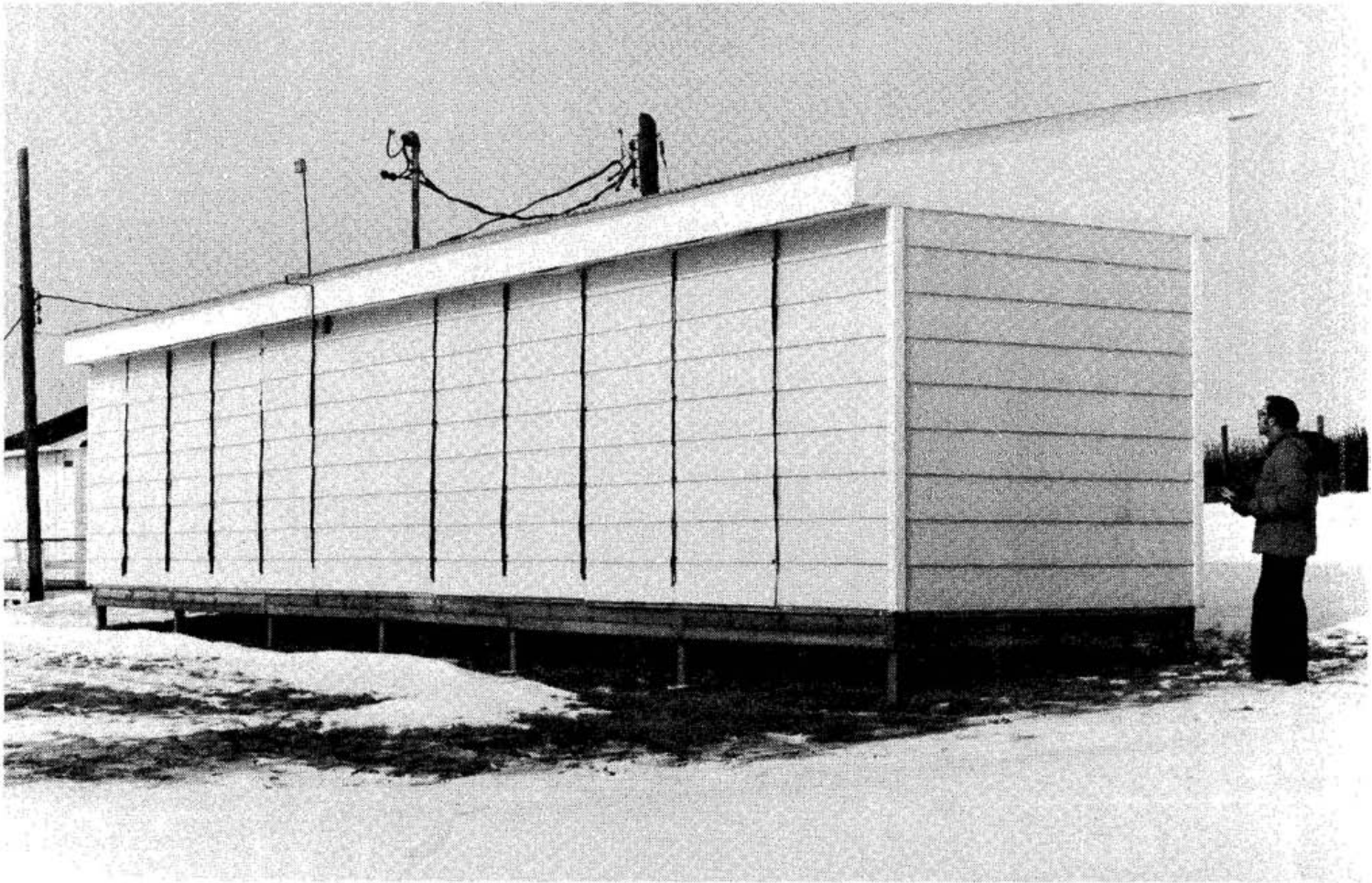
Figure 1. The test building at Valley View near Madison, Wisconsin.
