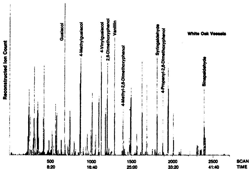
FIGURE 4.--Pyrogram of white oak vessels.
