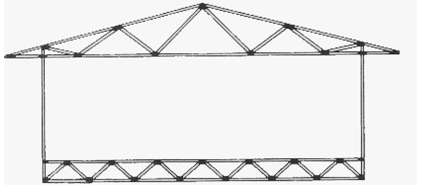
STRENGTH —The truss-framed system combined floor, walls, and roof into a unitized frame for structural continuity from the foundation up to the ridge.
