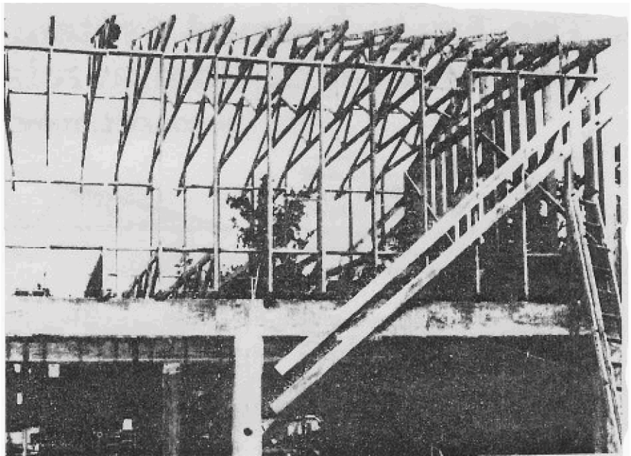
FAST—Florida Keys Truss, Inc., recently erected a 1500 square foot house in two hours and 50 minutes. It was built on an elevated concrete beam and pedestal foundation for protection from storm surge during hurricanes (Photo—Florida Keys Truss, Inc.)
