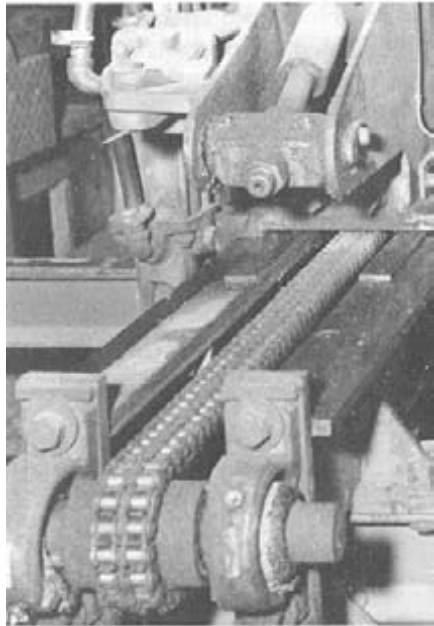
Figure 14.—Knees on this carriage are driven by a double roller chain from the set shaft.
