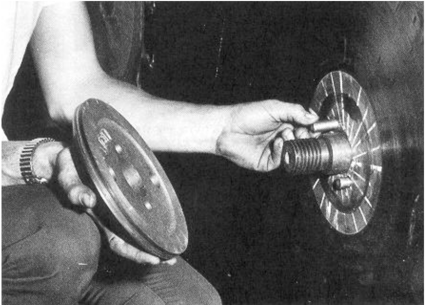
Figure 23.—Inspect lug pins for damage before replacing the collar and tightening the arbor nut.
