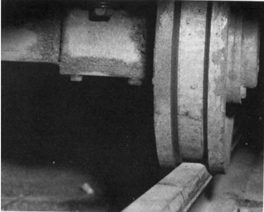
Figure 54. – A proper fit between the guide wheel and rail is evidenced by the wheel riding the bevel of the rail without the bottom of the wheel end the top of the rail making contact.
