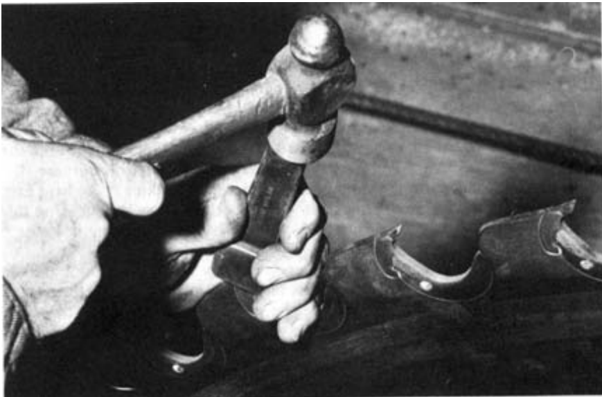
Figure 42. – Proper swaging requires positioning, holding, and striking the swage correctly.
