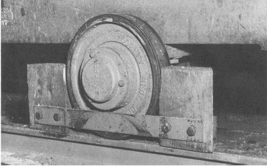
Figure 19.—Well designed track cleaners are essential in keeping debris off the tracks as well as the wheels.
