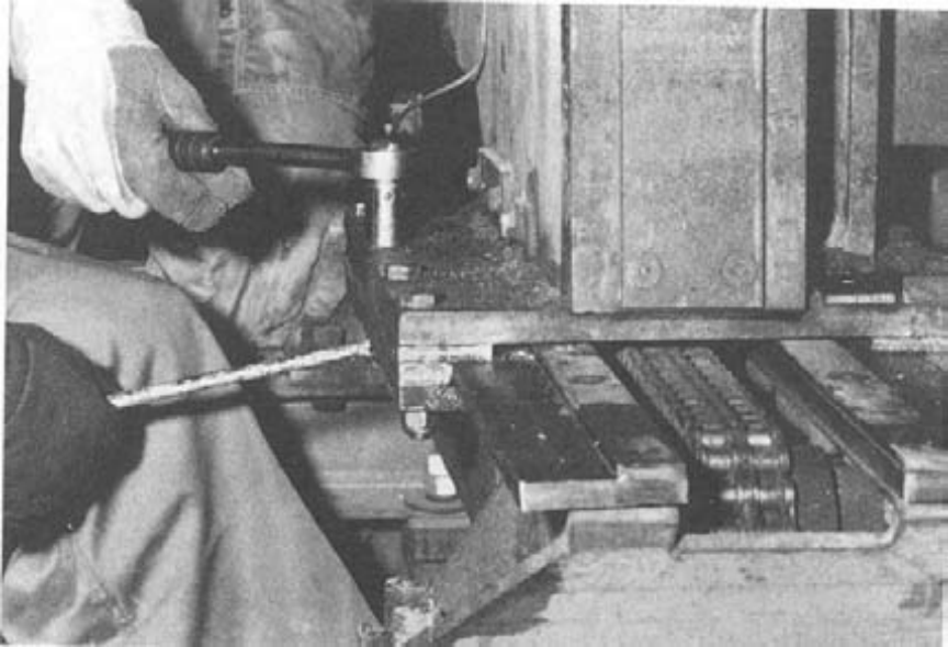
Figure 13. – Adjust shim strips between sliding surfaces of the headblock and knee to remove slack.
