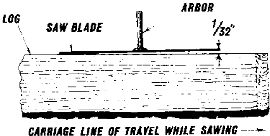
Figure 21.—Lead is put into saw by adjusting the arbor so that backside of the saw is offset approximately \frac{1}{32} inch relative to the line of carriage travel.
