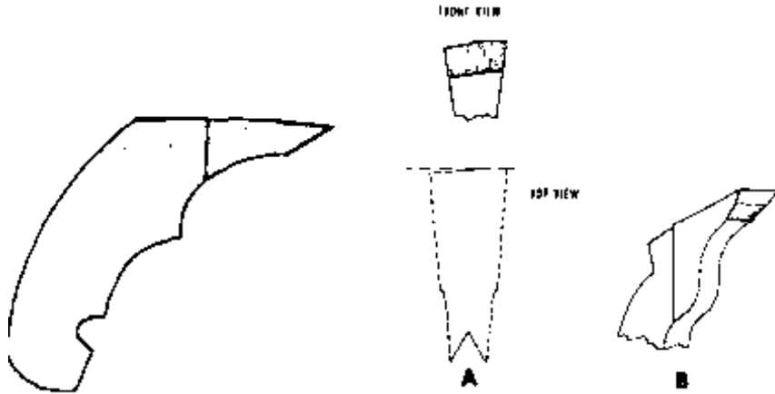
Figure 39. – Avoid excessive top filing as it lowers the cutting edge and reduces top clearance, thereby inhibiting carriage feed and increasing power consumption.
