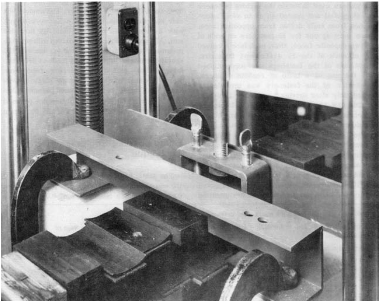
Figure 3.--Method of clamping and supporting test specimen for static withdrawal tests. Thumb screws clamp steel backup plate to cover piece to minimize bending of cover piece during withdrawal. Specimens have been stored outdoors for 1 year.
