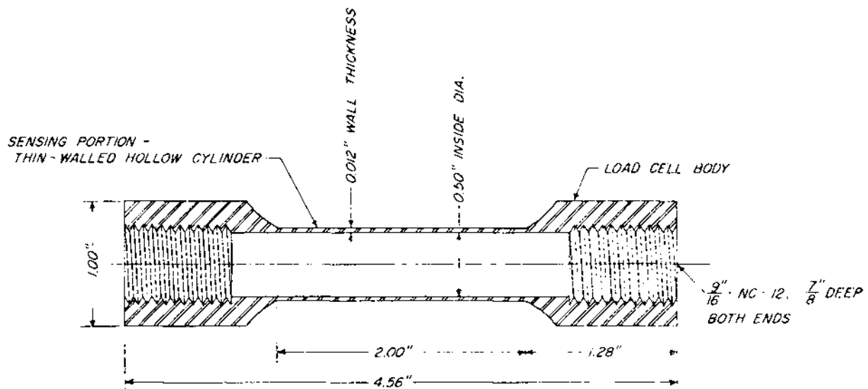
Figure 5.--Sketch of load cell.
