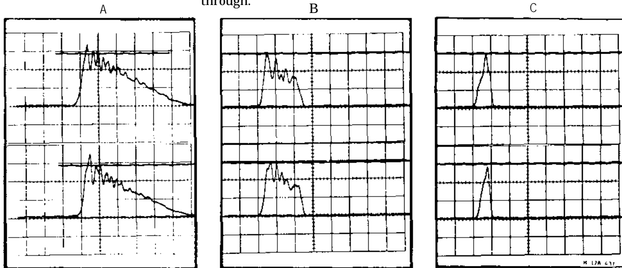
Figure 6.--Typical traces of dynamic withdrawal of fasteners: A , fastener pulled out (approximate distance 1-3/4 inches); B , fastener pulled through white pine cover piece (approximate distance 3/4 inch); C , fastener pulled through plywood cover piece (approximate distance 1/4 inch). Parallel horizontal traces are calibration lines and represent 370 pounds. Each grid is 1 centimeter and horizontal travel of trace is 20 milliseconds per centimeter. Duration of pulse is influenced by the distance fastener is withdrawn or pulled through.
