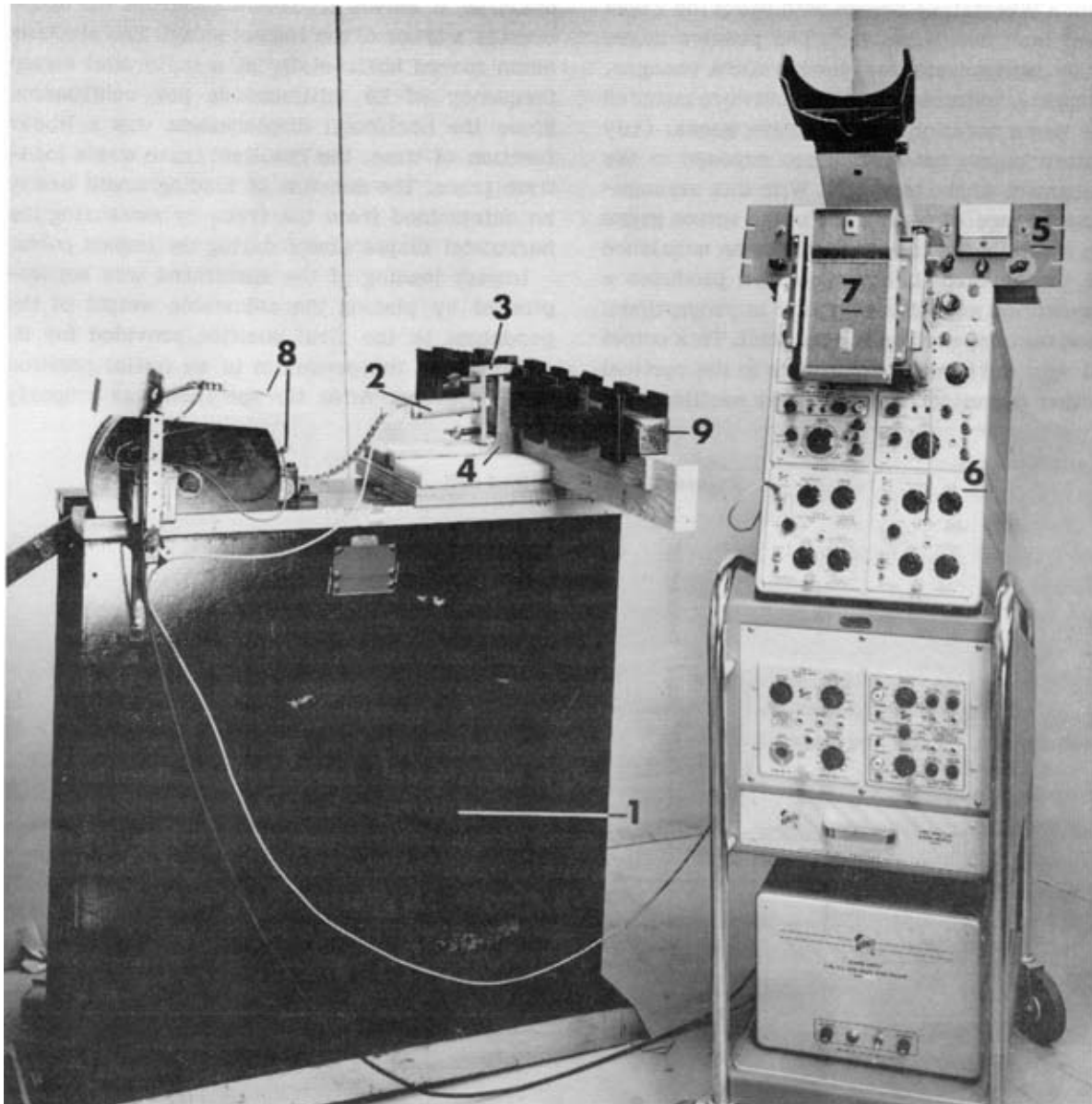
Figure 4.--Equipment for conducting dynamic withdrawal test of fasteners in simulated container application. (1), FPL toughness machine; (2), resistance type strain-gage load cell; (3), clamp; (4), test specimen restraining supports; (5), calibration box; (6), cathode ray oscilloscope; (7), Land process camera; (8), triggering device; and (9), test specimen.
