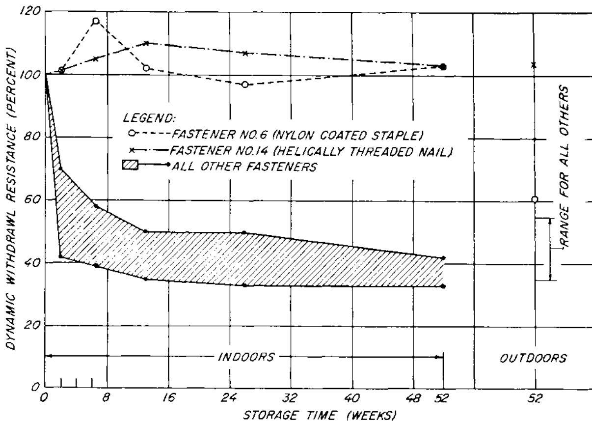
Figure 10.--Effect of storage time on dynamic withdrawal resistance of fasteners. Indoor storage maintained at 73° F. and 50 percent relative humidity. Fastener description: No. 6 , 16 gage (0.0625 in.), 7/16-in. crown, 2-in. leg, nylon-coated staple through 1/4-in. plywood; No. 14 , 0.100- by 2-1/4-in. helically threaded nail through 3/4-in. white pine.
