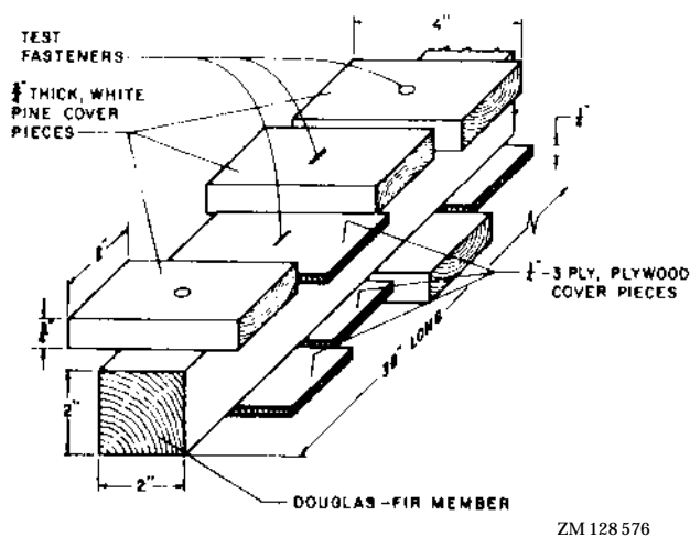
Figure 1.--Arrangement and details of test specimens. Fasteners are located 2-1/4 in. on center, and staggered 1/2 in. Top and bottom locations are offset to avoid interference.
