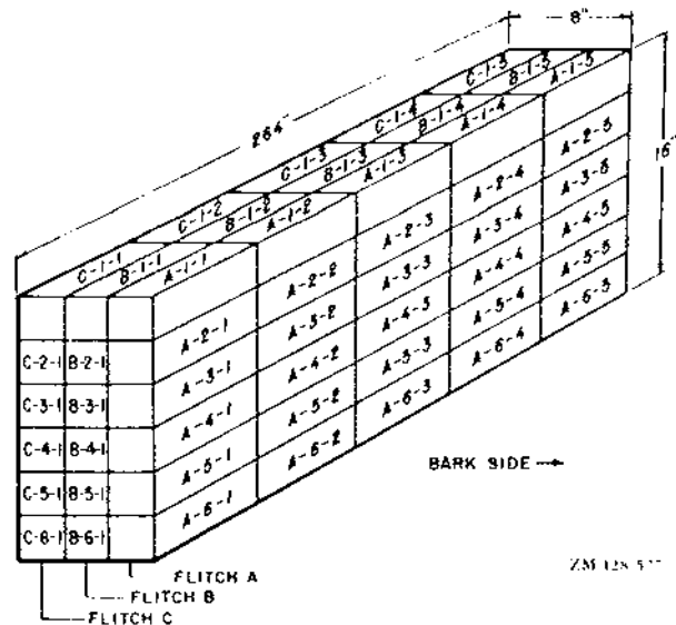
Figure 2.--Numbering system and method of cutting timber to obtain test specimens.
