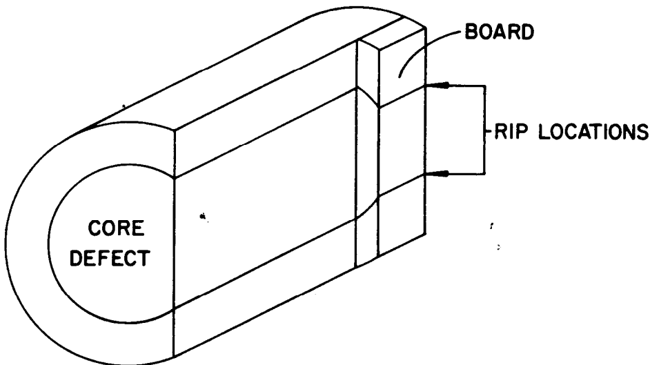
Figure 9. Cut away view of a log showing how the rip location in ripping for grade is referenced to the core defect on the outer face of the board. The kerf is taken out of the core defect. (M 148 330)
