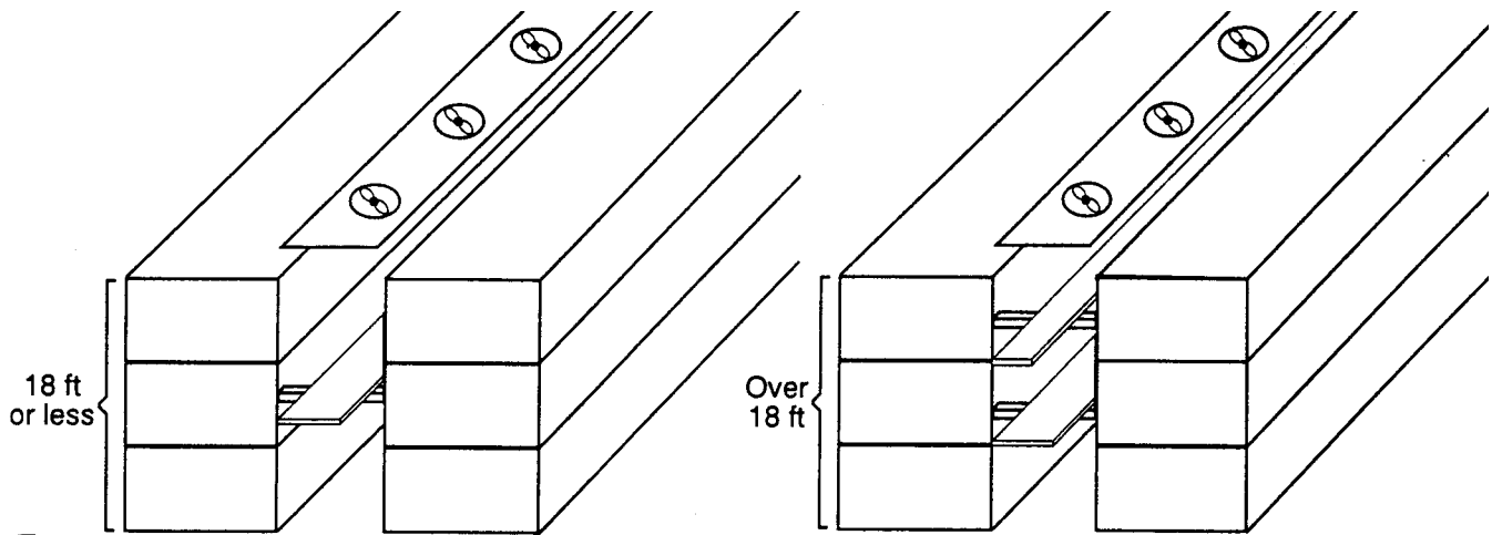
Figure 2. Placement of baffles in plenum space.
