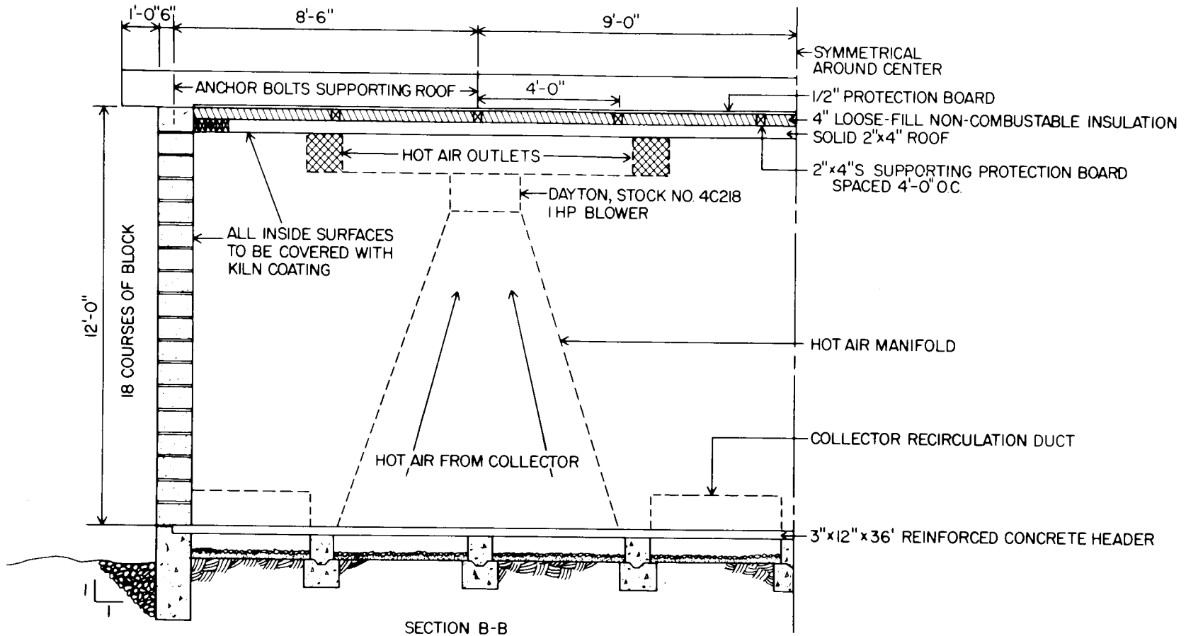
Figure A-5.—Section view of solar collector ducts. (ML845654)
