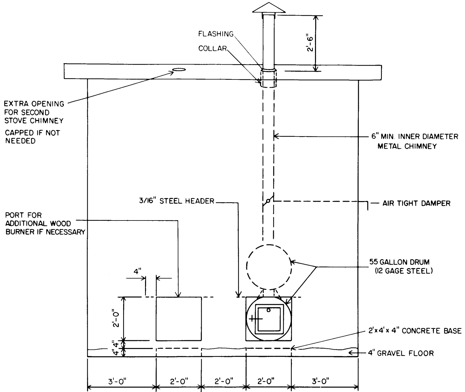
REAR ELEVATION : FURNACE ROOM
