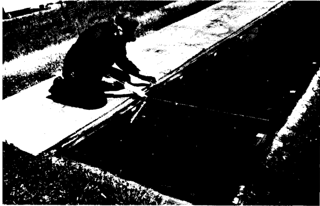
Figure 2.—Glass collector cover on prototype kiln. Wood sills shown in this photo are not included in the design of the 6,000-fbm kiln. (M830178-8)
