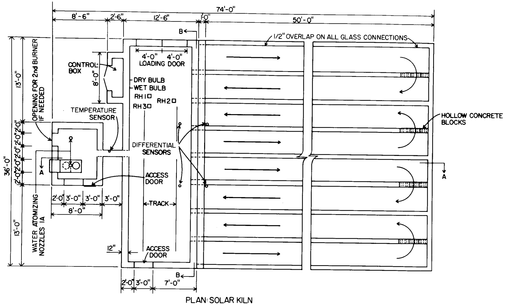
Figure A-3.—Plan view of solar/wood residue kiln. (ML845653)
