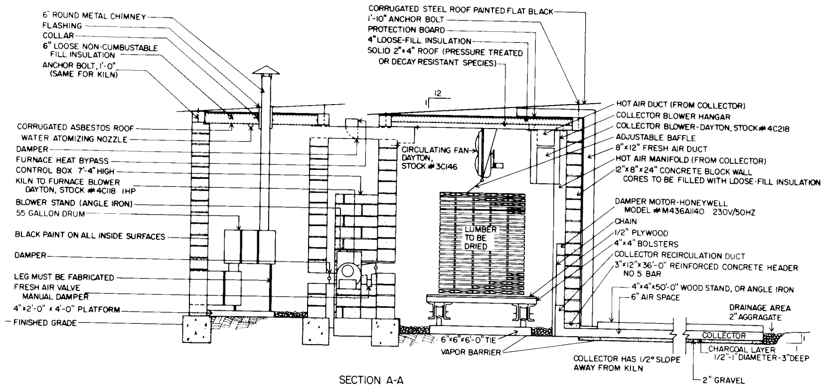
Figure A-4.—Section view of solar/wood residue kiln. (ML845652)
