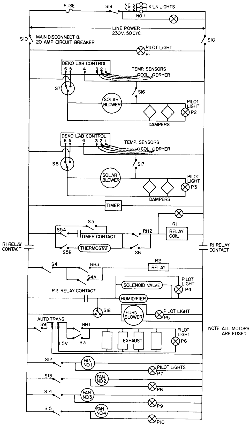
Figure A-8.— Wiring diagram of control system. (ML845650)
