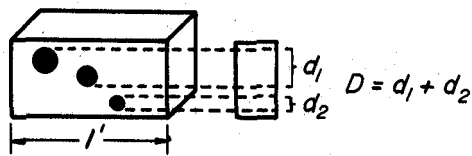
Figure 7.—Assumed cross-sectional area of knots in 7-foot interval of unit depth projected on end of the interval.
